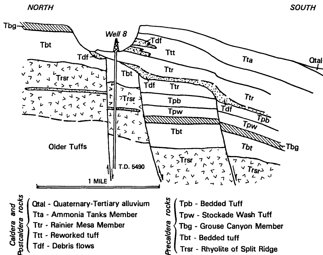
Fig. 20. Sketch of geologic relations at Well 8 (Stop 15).
